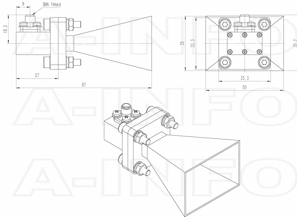
SMA-Female Output (P/N: LB-62-15-C-SF)
