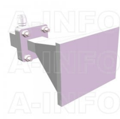
LB-62-15-C-TFSPO Standard Gain Horn Antenna 12.4-18GHz 15dB Gain TNC Female
