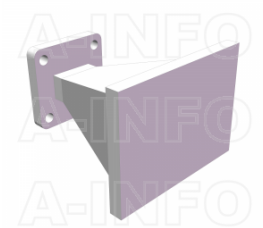
LB-62-15-ASPO Standard Gain Horn Antenna 12.4-18GHz 15dB Gain Rectangular Waveguide Interface
